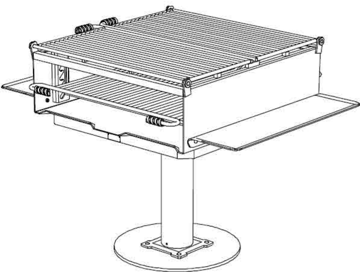
STANDARD B8 SURFACE MOUNT INSTALLATION
