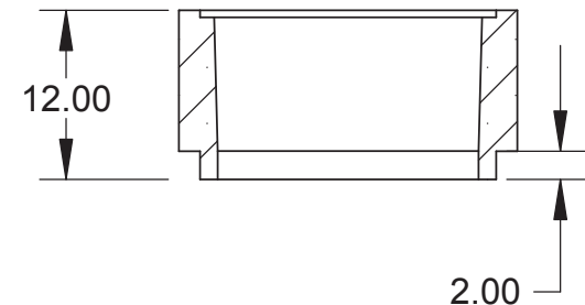
SECTION B-B SCALE 1:15
