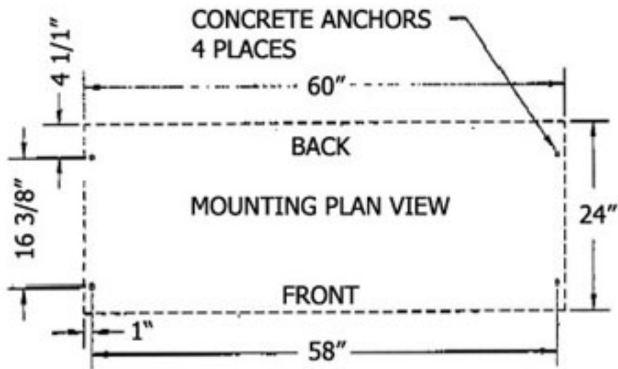
DIAGRAM 4: BENCH 5 FOOT LENGTH 251-1004, SURFACE MOUNTING
