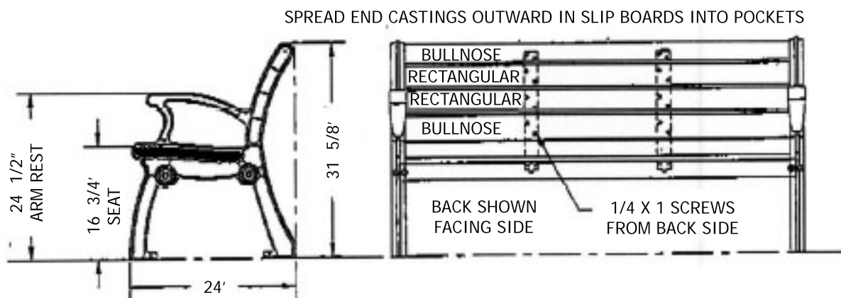
DIAGRAM 3: PLACING AND FASTENING "BACK" BOARDS IN PLACE 251-1004
