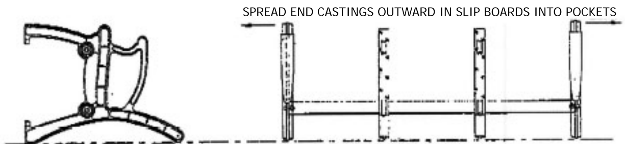
DIAGRAM 1: END CASTING AND SUPPORT TUBE ASSEMBLY 251-1004 BENCH
