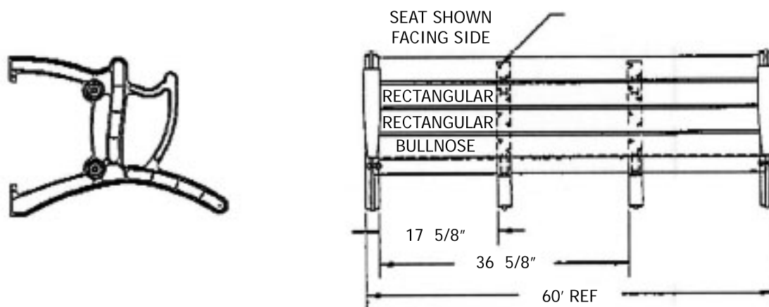
DIAGRAM 2: PLACING AND FASTENING "SEAT" BOARDS IN PLACE 251-1004
