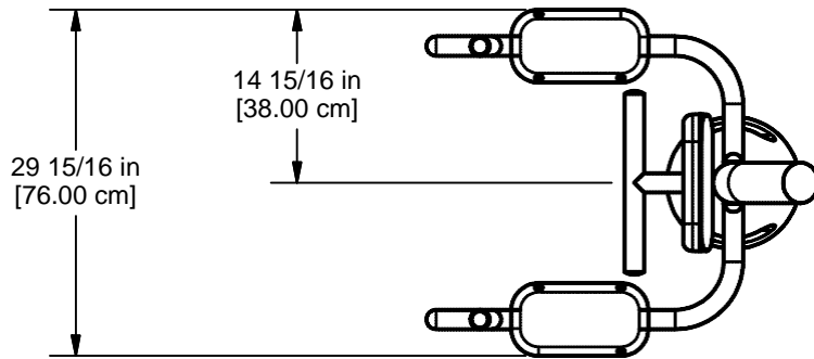
PLAN VIEW (SURFACE)
