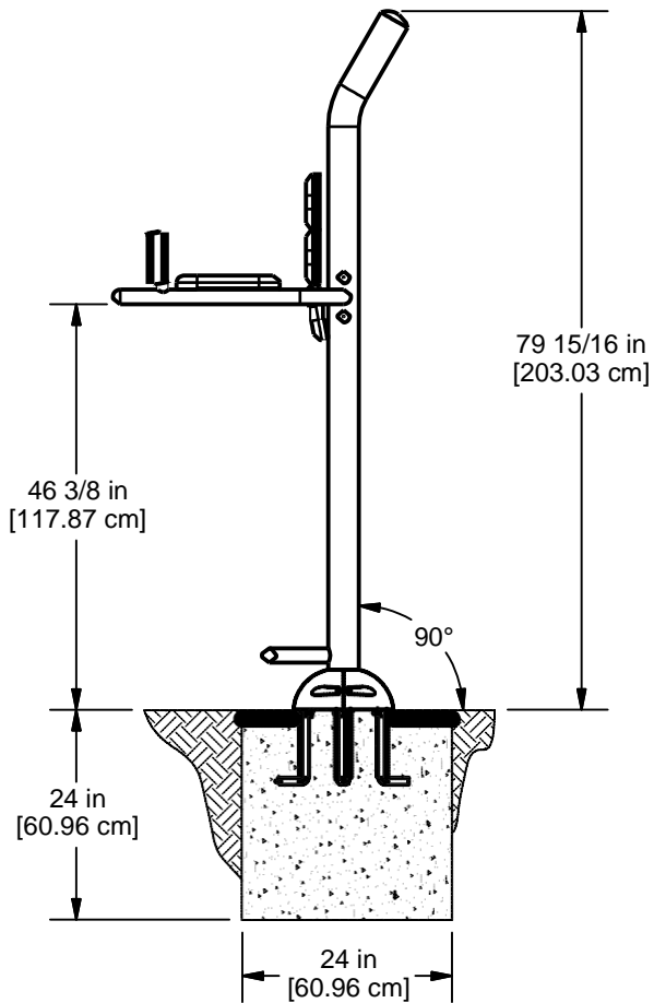
ELEVATION VIEW (FOOTING)
