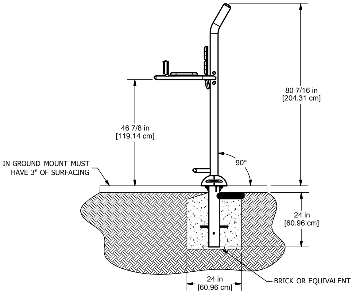
ELEVATION VIEW (IN GROUND)
