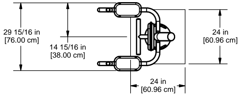
PLAN VIEW (IN GROUND)
