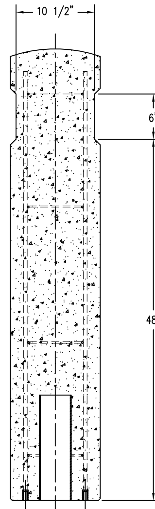
4 CROSS SECTION
