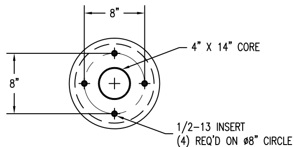
3 BOTTOM VIEW
