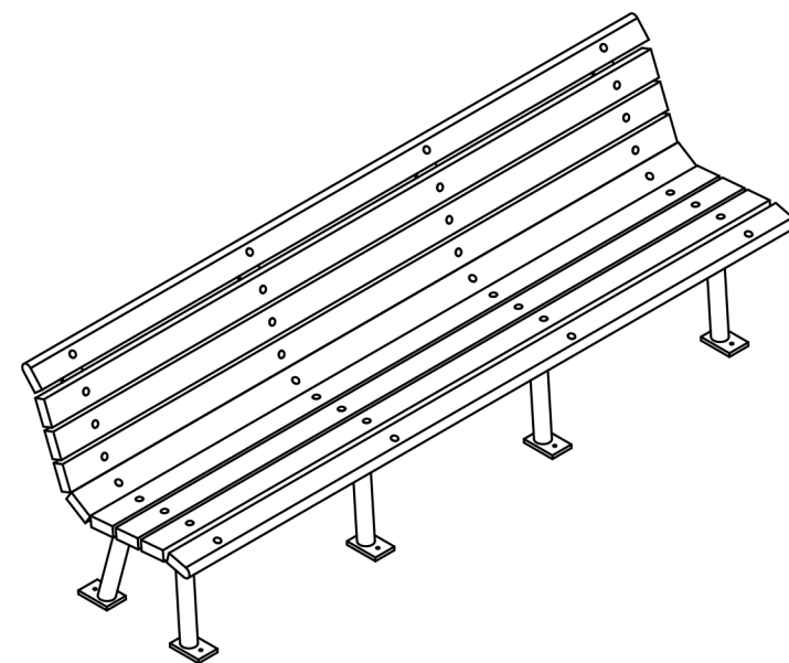
3D ISOMETRIC VIEW
