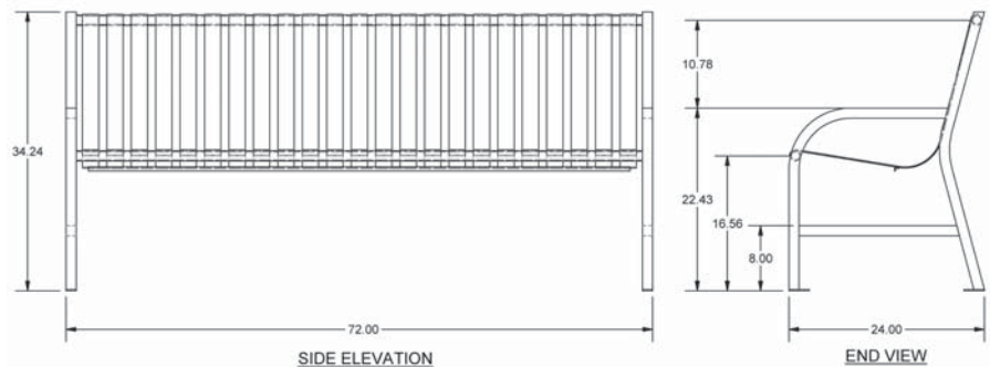
SIDE ELEVATION
